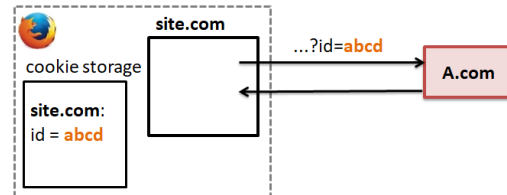
Fig. 10. Analytics behavior.
